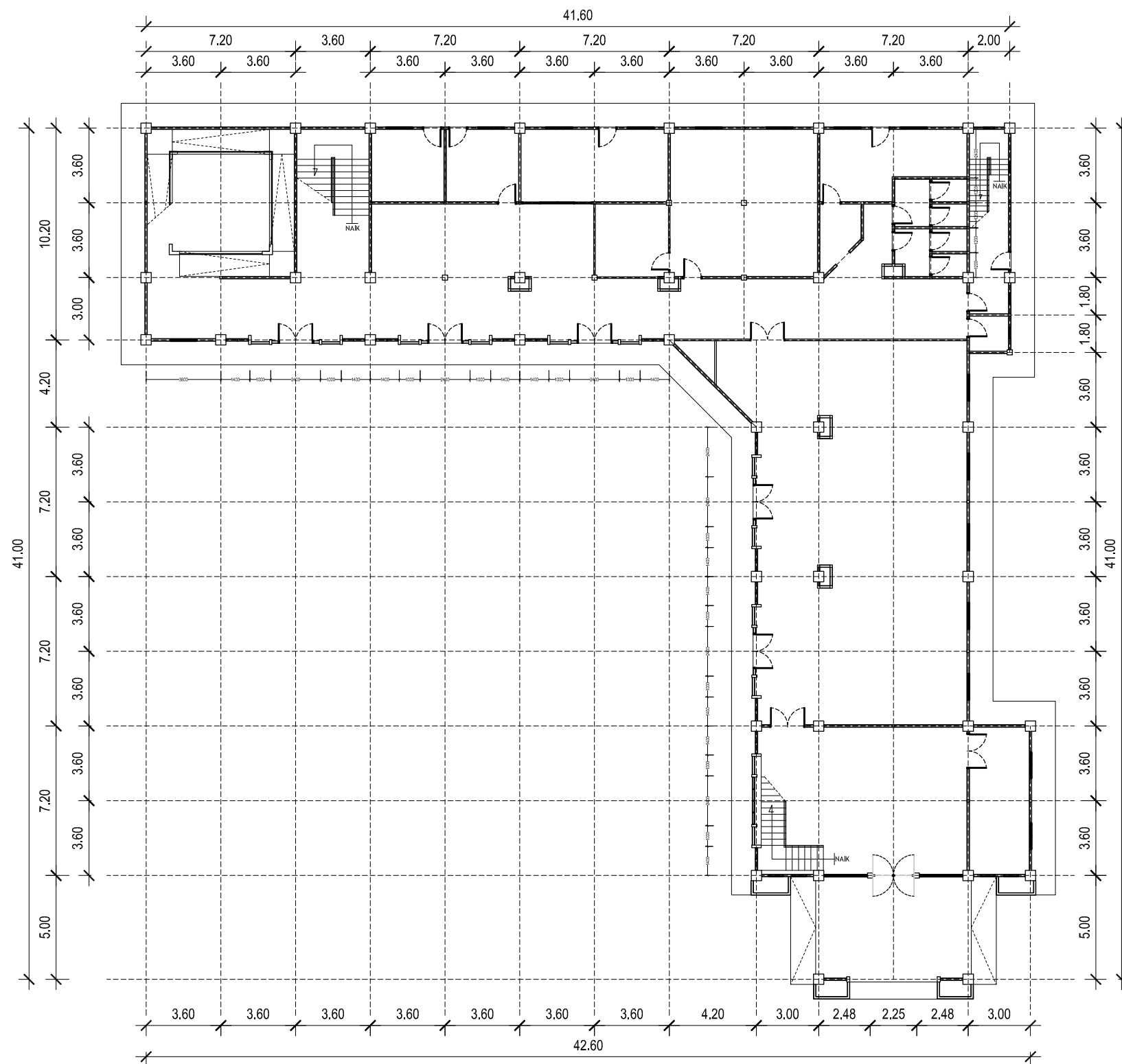
1 DENAH LANTAI 1 EKSISTING ARS SKALA 1 : 250
