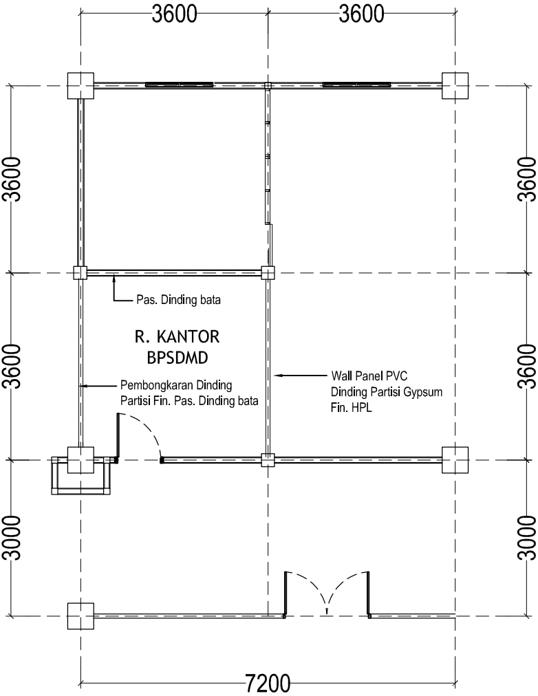
1 ARS DENAH R. KANTOR BPSDMD LT. 1 S K A L A 1 : 100
