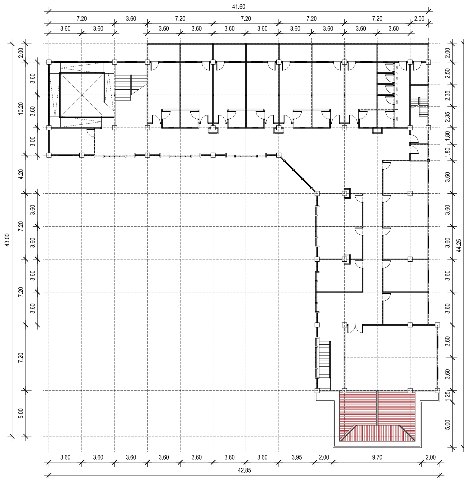
1 ARS DENAH LANTAI 2 EKSISTING SKALA 1 : 250
